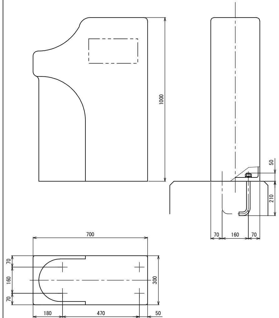
OK-G4-100 材質：鋳鉄
